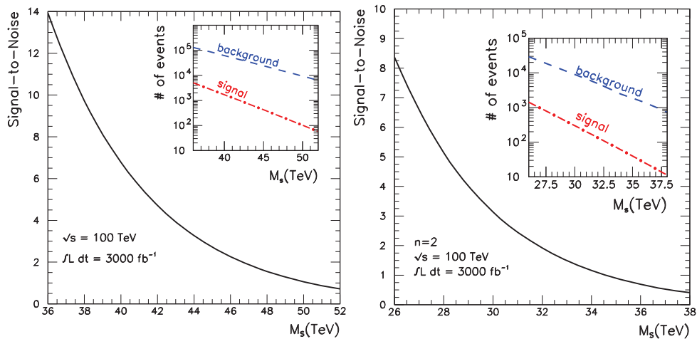
Fig. 3 – Dijet signal-to-noise ratio of the lowest n = 1 (left) and n = 2 (right) Regge excitations for a future 100 TeV hadron collider.
