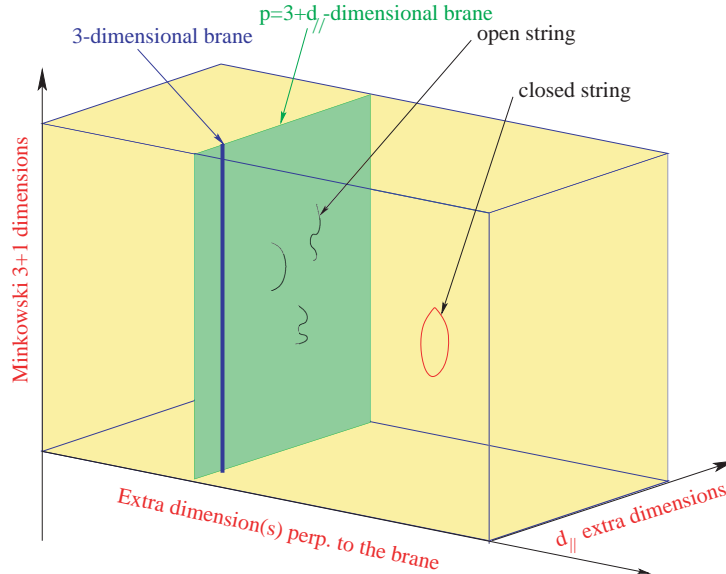
Fig. 1 – D-brane world universe in type I string framework.
