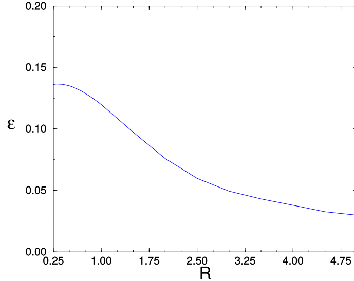
Fig. 4 – The coefficient \varepsilon of the one loop Higgs mass (13).
