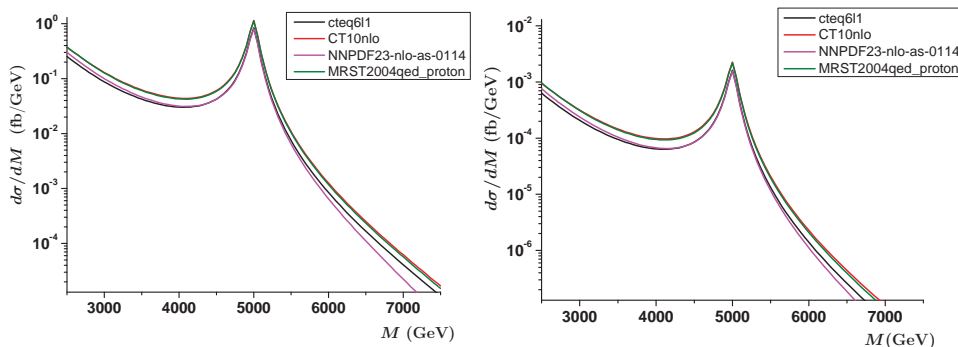
Fig. 2 – Production of the first Regge excitations at LHC in the dijet (left) and \gamma + \text{jet} (right) channels, for M_s = 5 \text{ TeV} . The cross-section is plotted as a function of the invariant mass M .
