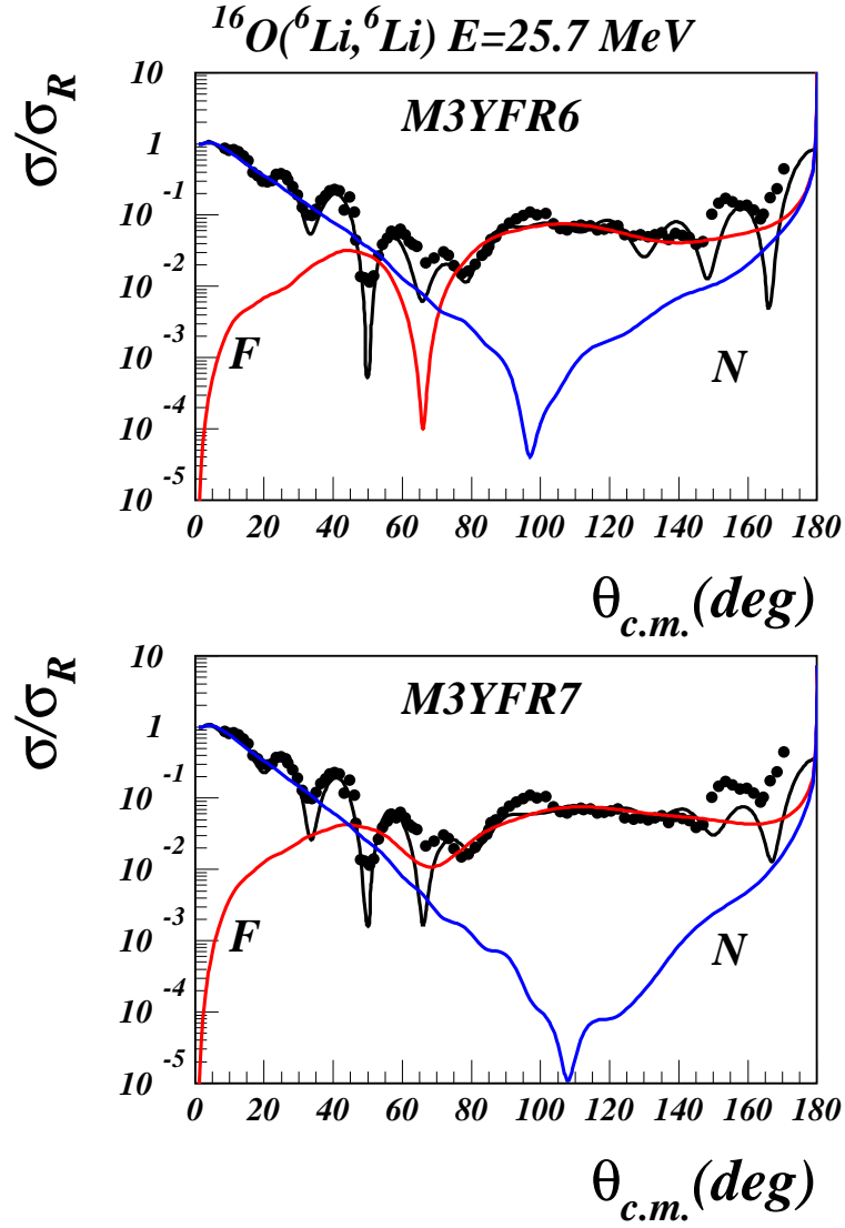
Fig. 9 – (Color online) Cross sections calculated with the finite range version of the M3Y effective interaction. Renormalization parameters and ranges are given in Table 3.
