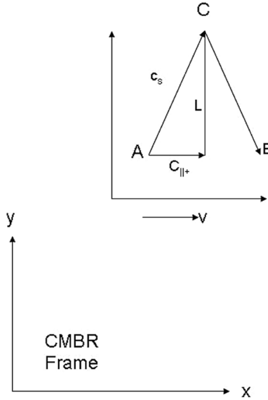
Fig. 1 – The Michelson-Morley experiment.
